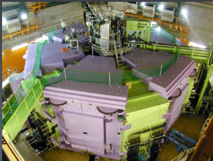
史上最も高性能な超伝導リングサイクロトロン。RIBFでは光速の約70%まで重イオンビームを加速できる。The Superconducting Ring Cyclotron with the highest performance in history, is able to accelerate very intense all-element heavy ions to a speed of about 70% of the velocity of light.
